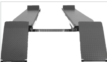
Profilift 2.40 F 460 Plat- form VAS 5248
