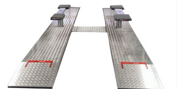
Masterlift 2.35 Combi Check in KA 1550 VAS 782 019
